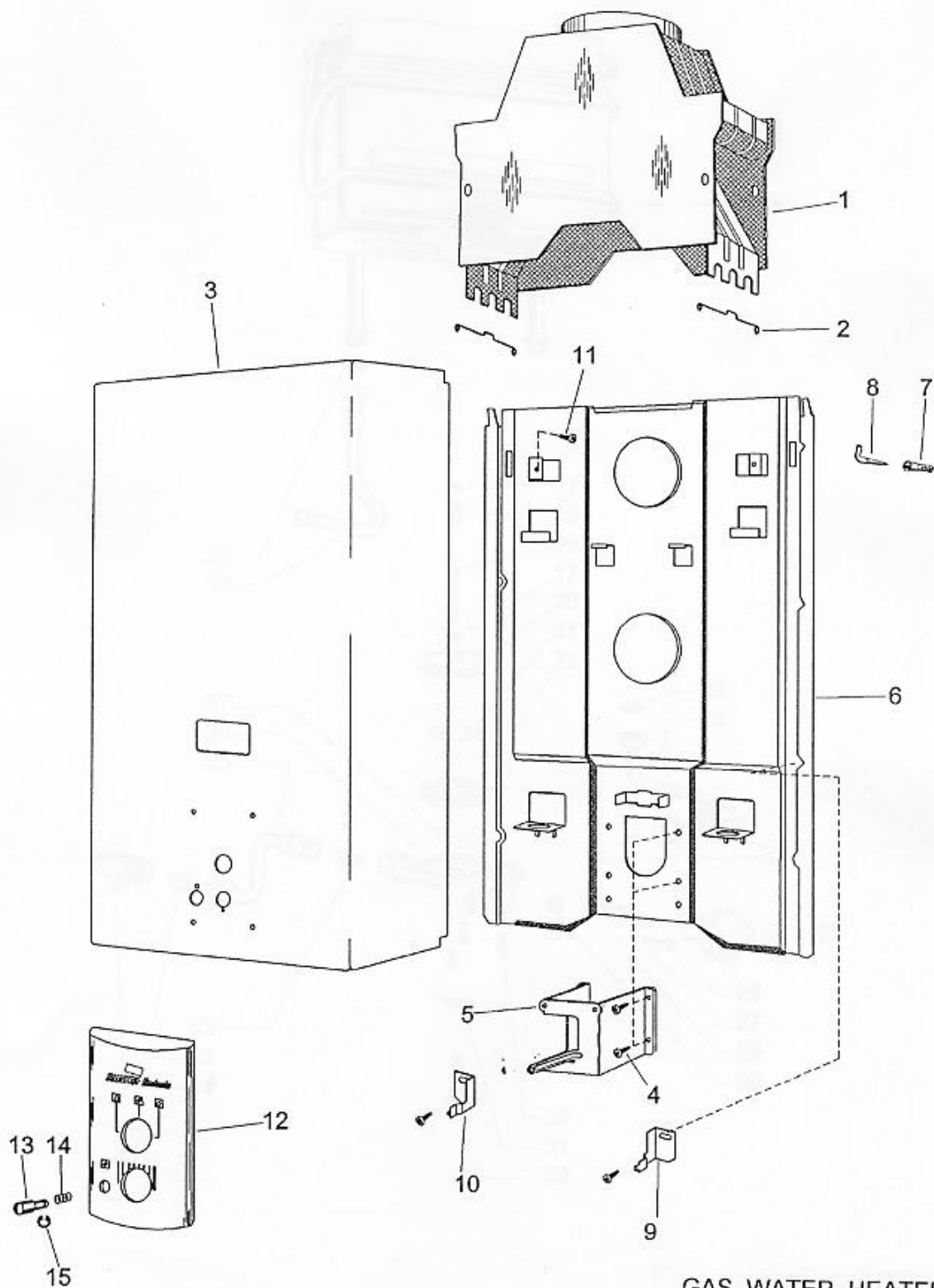
GAS WATER HEATER
